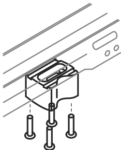
Rigid mounting KRG Chassis
