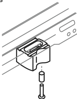
Swivel mounting KRG Chassis
